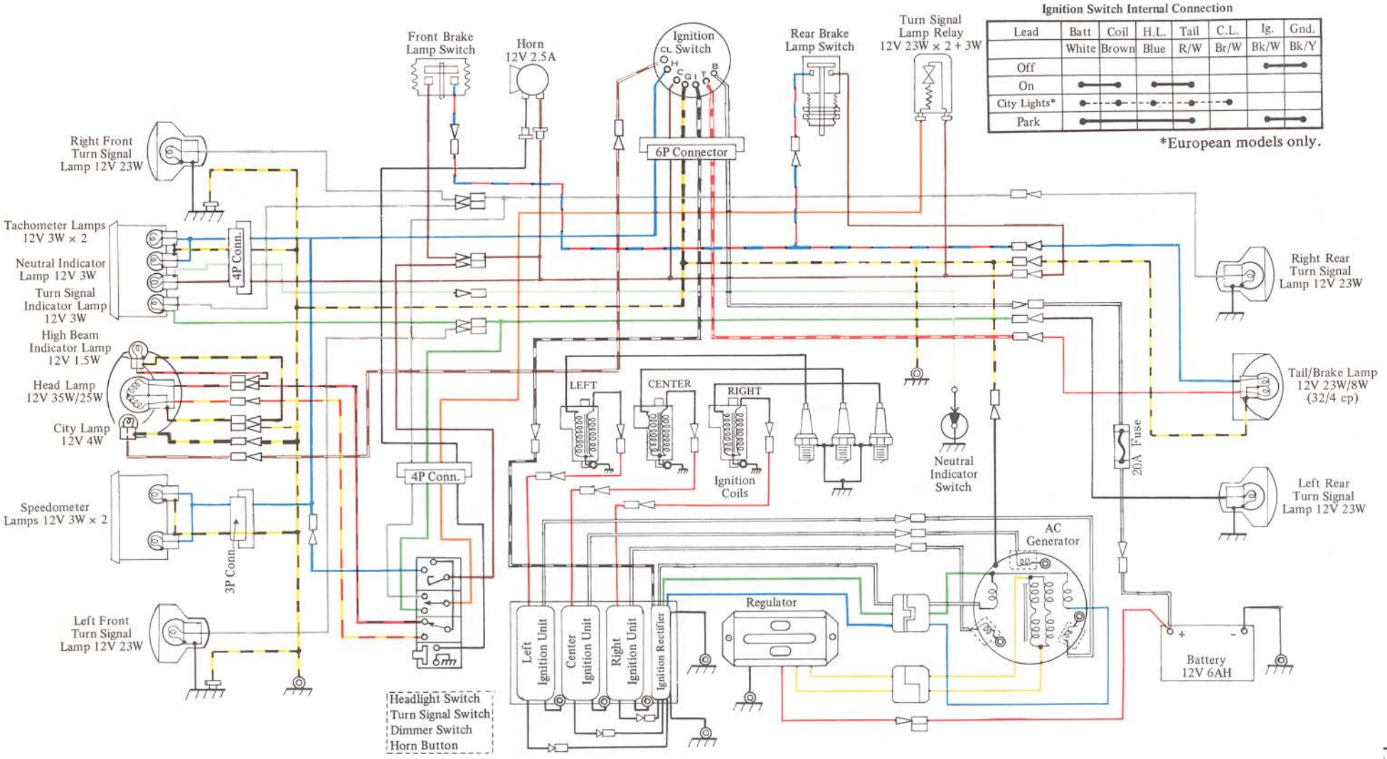
Ignition Switch Internal Connection
